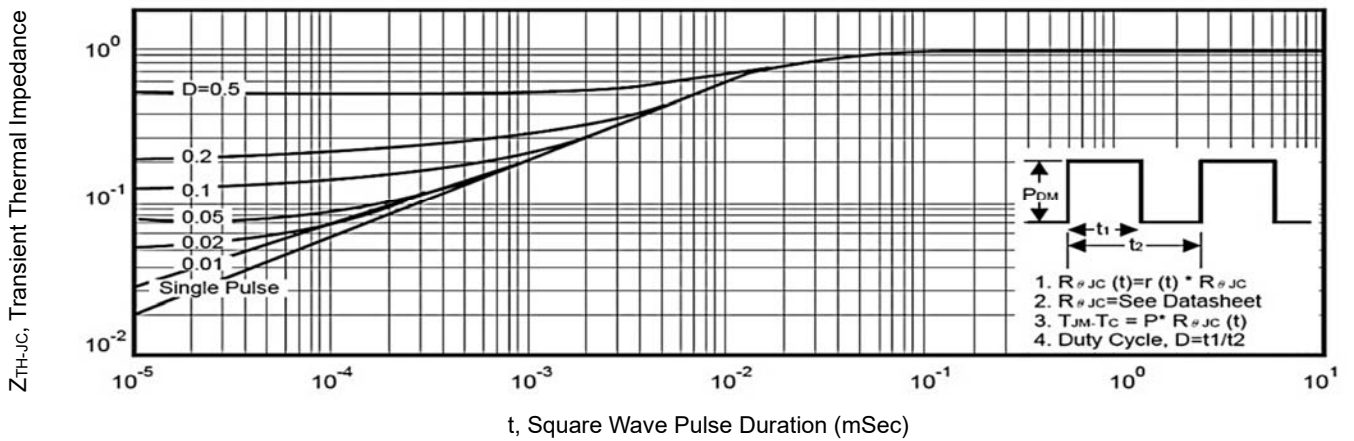
Normalized Transient Thermal Impedance Curve
